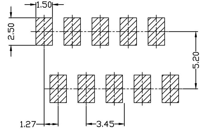
Recommended P.C.B Layout(Top Side)
