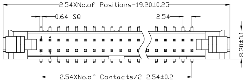
Long Latch (长耳) L1=8.00
